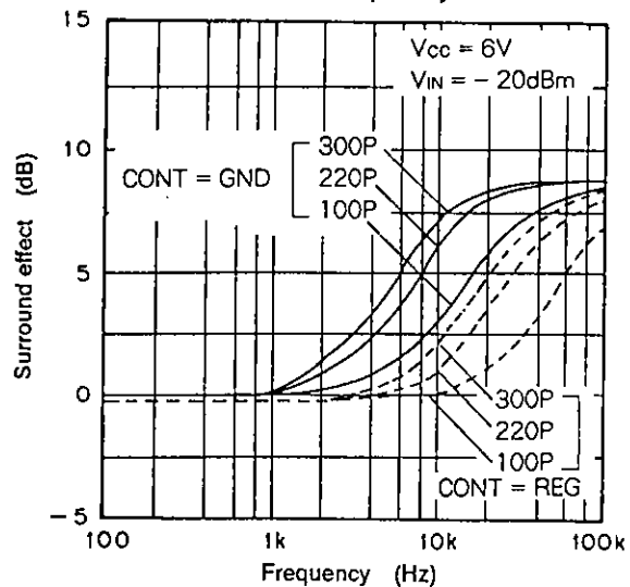
Surround effect vs. Frequency characteristics
